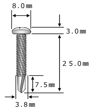
4×25
